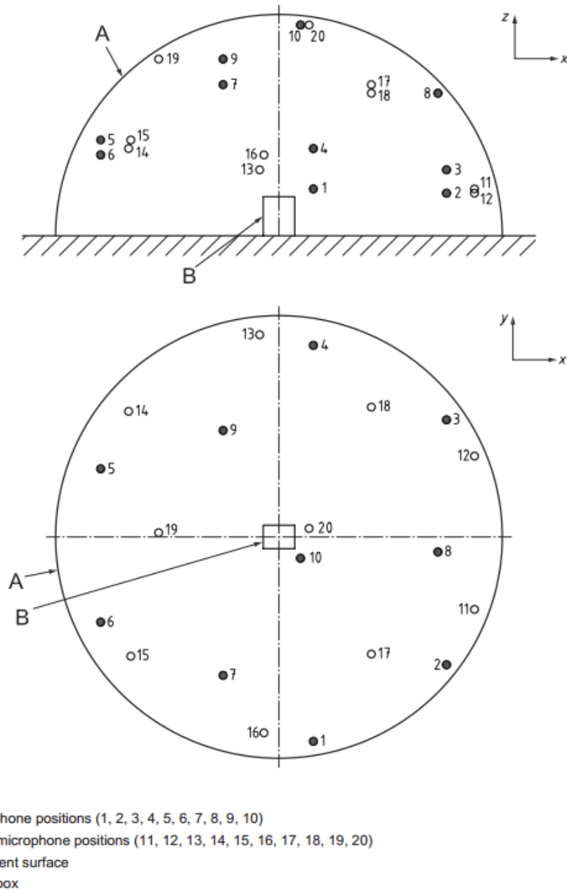
Figure 2: Microphone Positions
